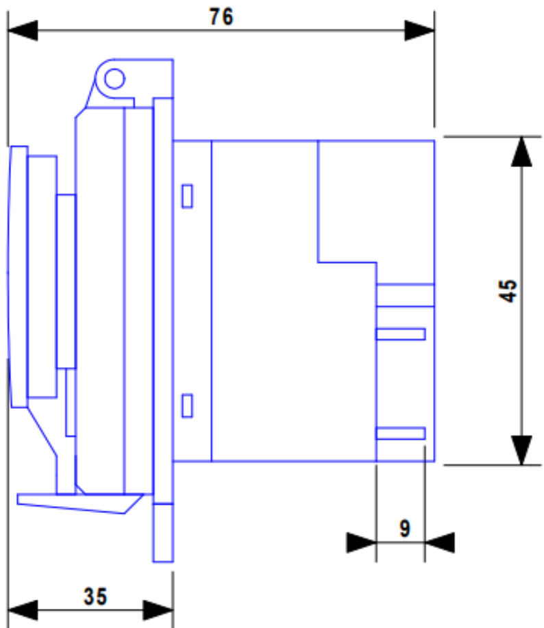
VISTA FRONTAL
